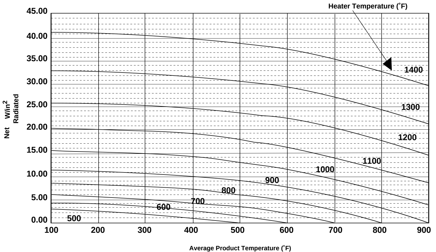
Stefan-Boltzman Equation (Fig. 7)
