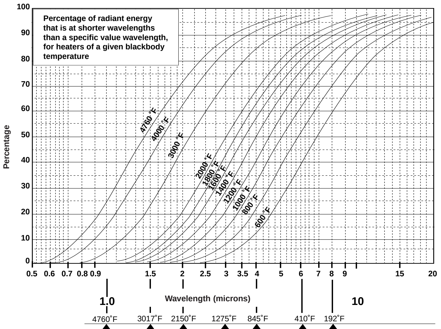
Radiant Energy Ratios For Several Blackbody Temperatures (Fig. 13)
