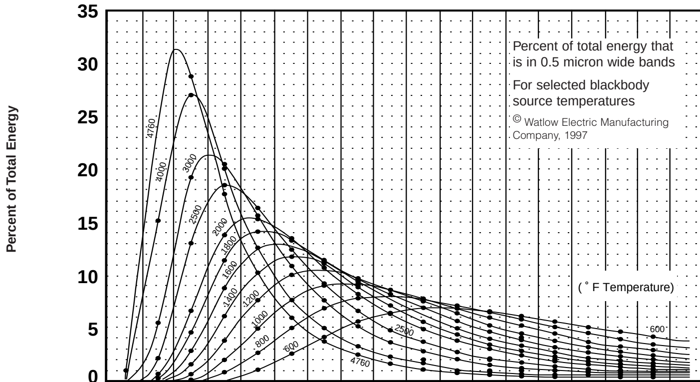
Blackbody Radiation By Micron Band Widths (Fig. 4)
