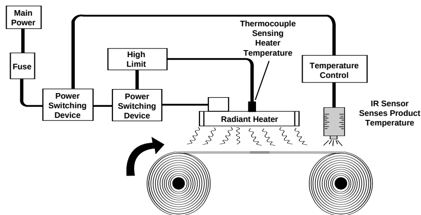
Product Temperature Sensed and Used to Control Heater Temperature
