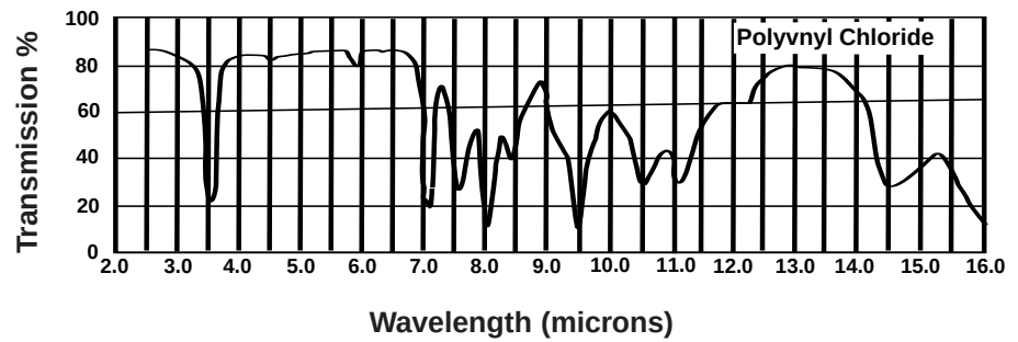
Transmission Spectrum for Polyvinyl Chloride (Fig. 14)
