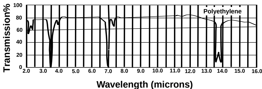
Transmission Spectrum for Polyethylene (Fig. 12)
