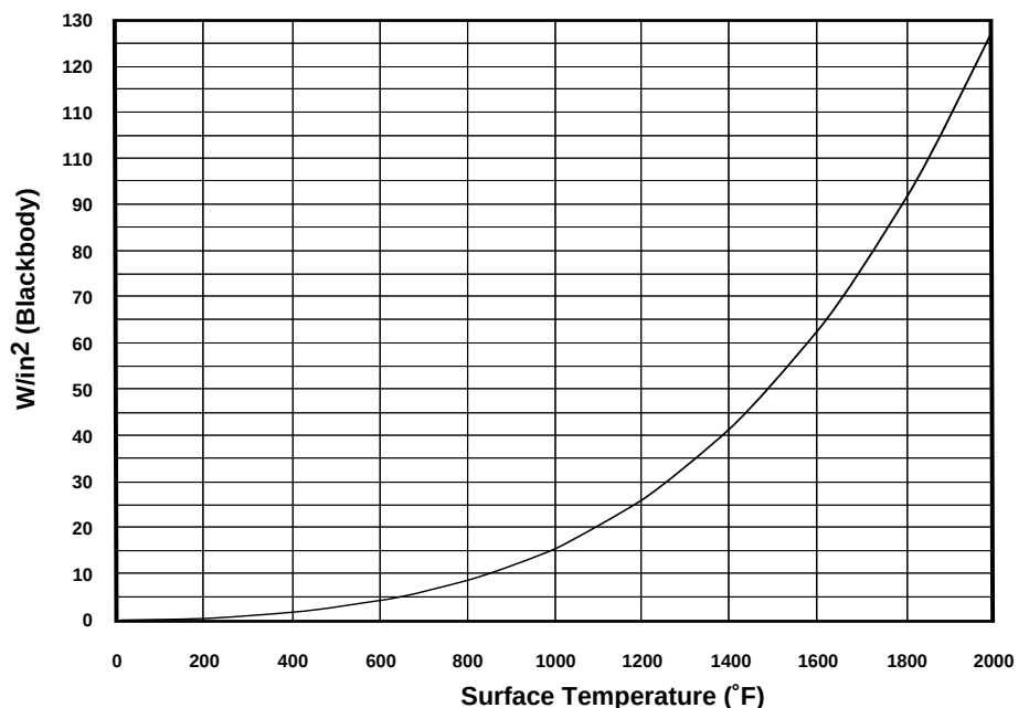
Radiated Power vs. Temperature (Fig. 6)
