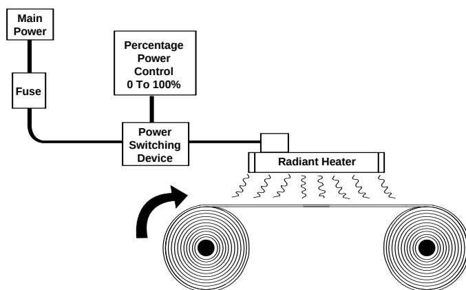
Open Loop: No Temperature Sensing
