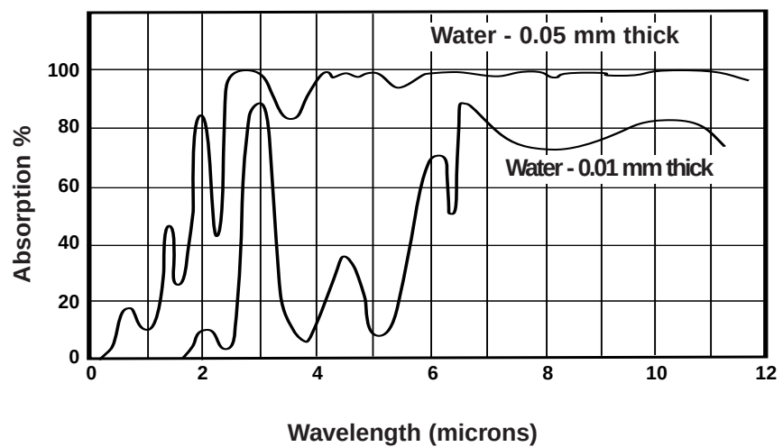
Spectral Absorption Curve For Water (Fig. 10)
