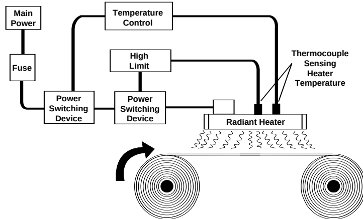
Closed Loop: Heater Temperature Sensed and Controlled
